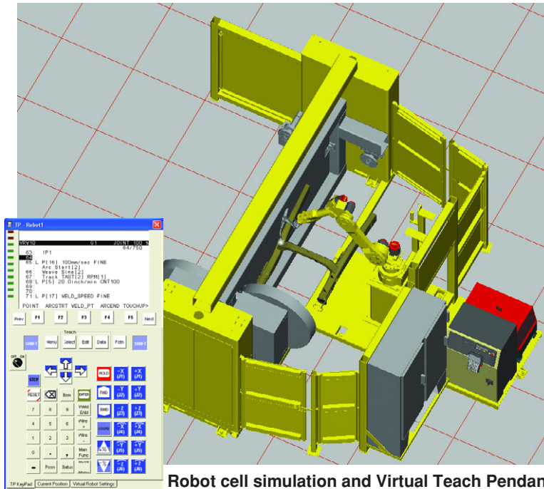
Robot cell simulation and Virtual Teach Pendant
